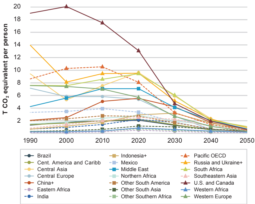
Figure 2.17: Fossil fuel CO 2 emissions in tonnes per capita, by region, under the BEA scenario
