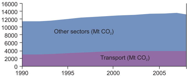
Figure 3.3: CO 2 emissions in megatonnes (Mt) from transport in 2008 (top) and change in CO 2 emissions from transport from 1990 to 2008, compared with other sectors (bottom)
